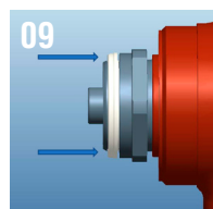
9.- Finish manually inserting the lip seal into the slot nozzle
